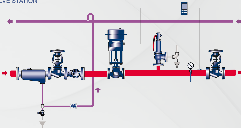
CONTROL VALVE STATION
