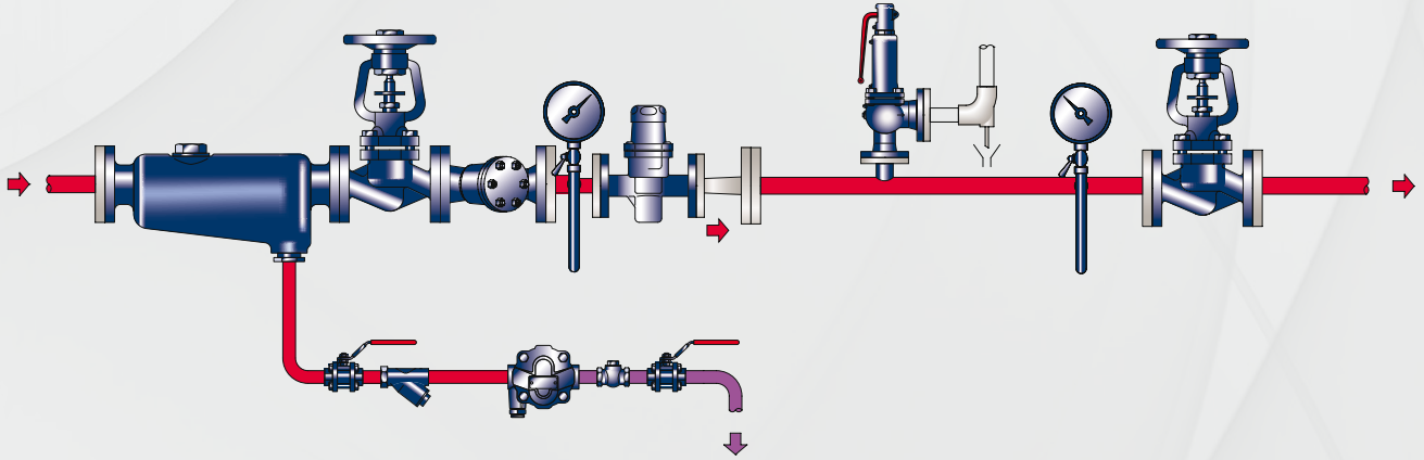
PRESSURE REDUCING VALVE STATION
