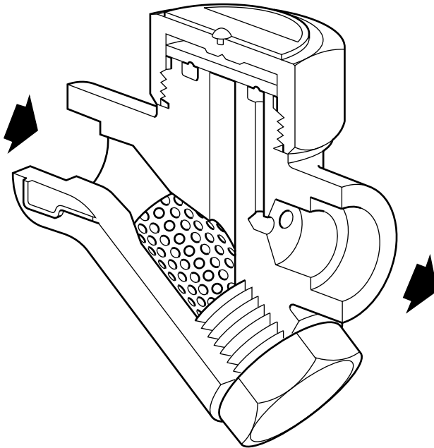
Fig. 1 TD42S3 thermodynamic steam trap
