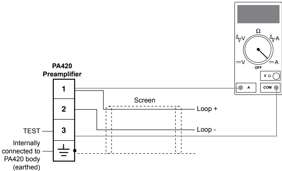
Fig. 6 Measuring the loop current (Please note that you don't need to disconnect the installation wiring)
