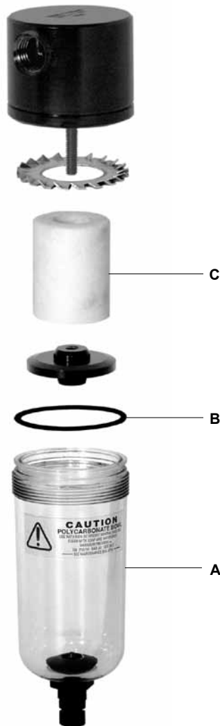
Fig. 5 Spare parts
