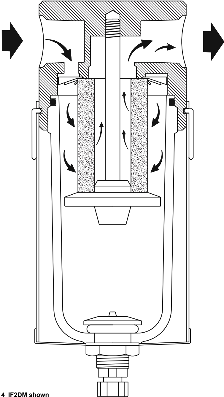
Fig. 4 IF2DM shown
