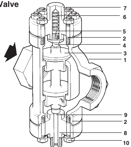
NSRA Valve
