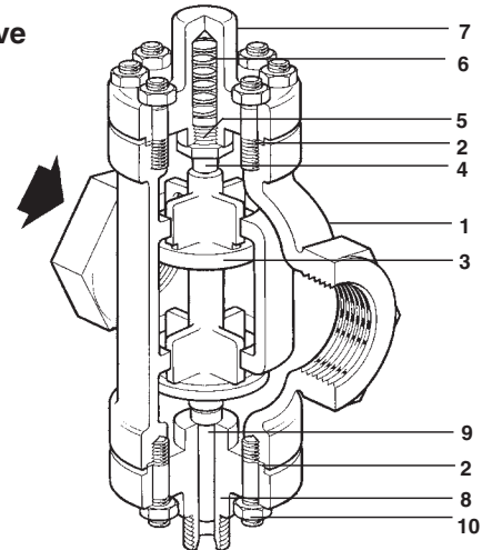
NSRA Valve
