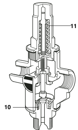
SBRA with fusible device and bleed
