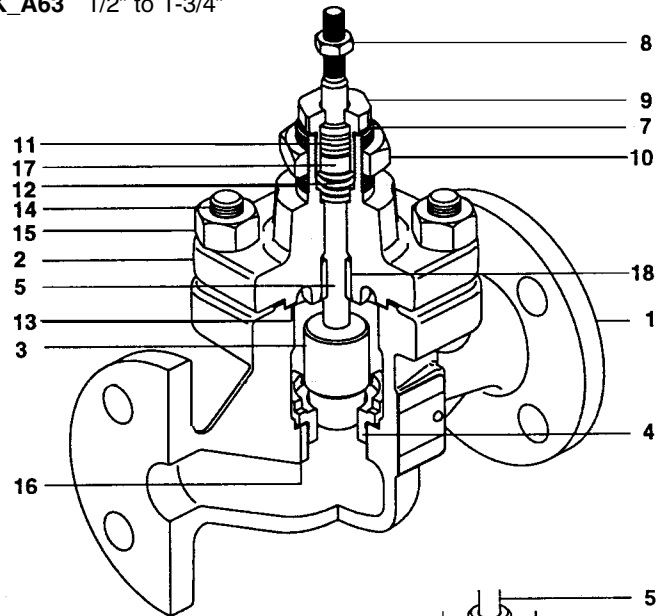
K_A63 1/2" to 1-3/4"
