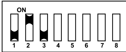
Fig. 7 Range 1000 - 9990 ( \mu\text{S/cm} or ppm)
