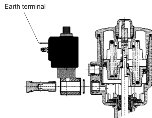
Fig. 5 DM solenoid valve mounting (Normally closed valves)
