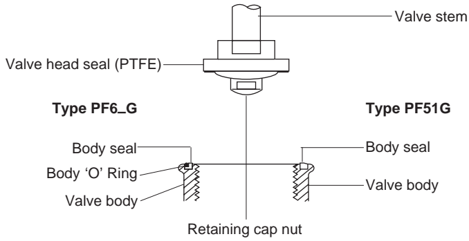
Fig. 8 BD (Bi-Directional) valves
