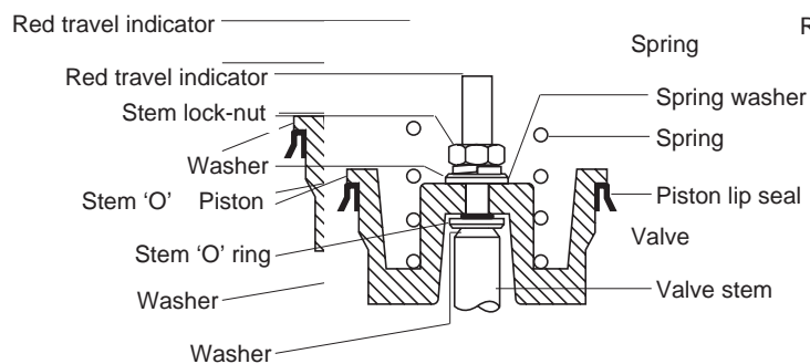
Fig. 6 NC (Normally Closed) valves
