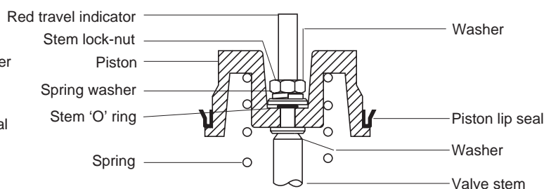
Fig. 7 NO (Normally Open) valves
