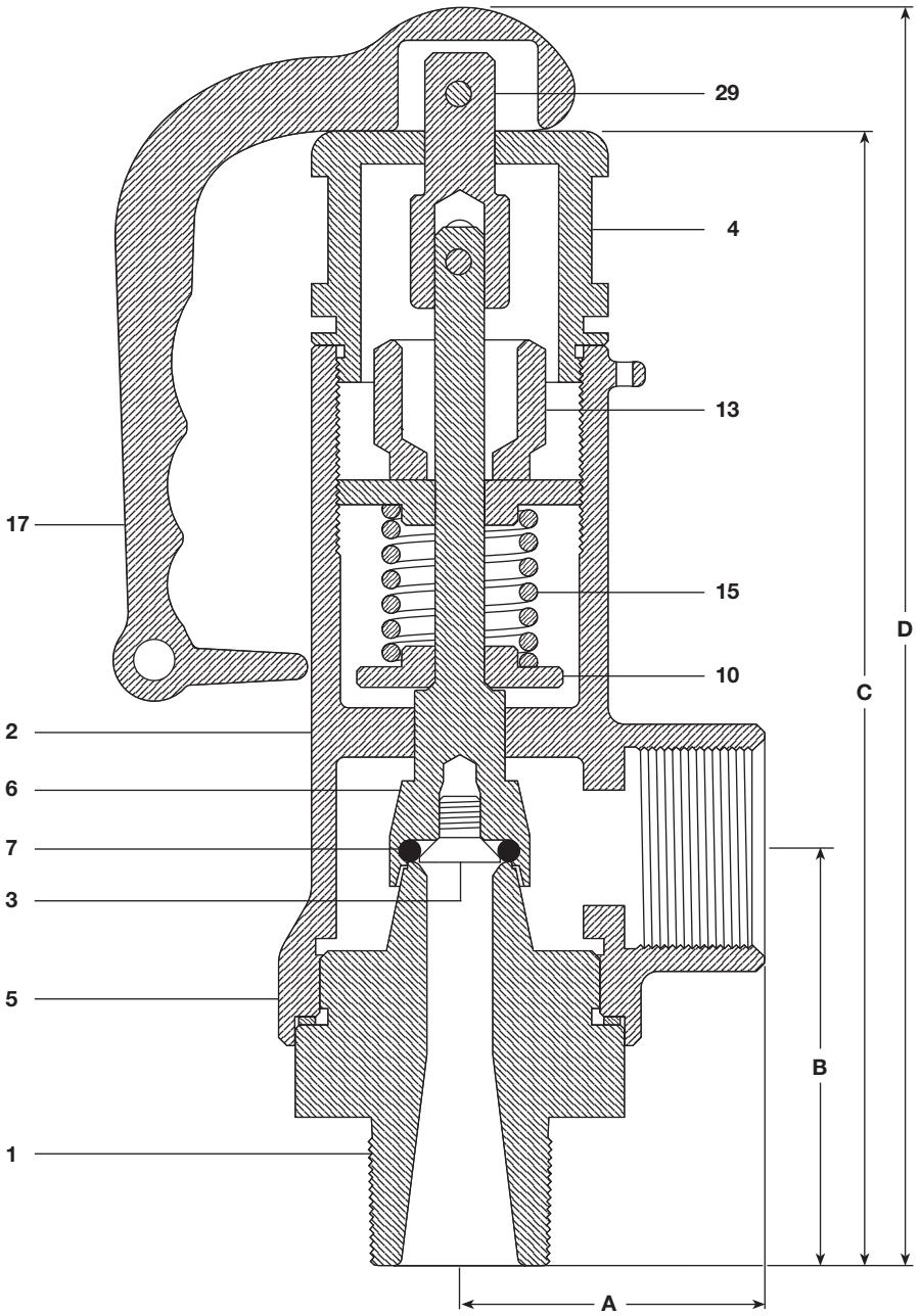
Fig. 2 SV405, SV405X and SV406 parts and dimensions
