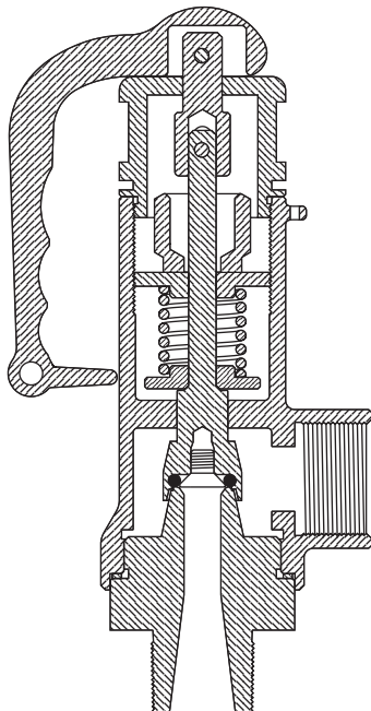
Fig. 1 SV405, SV405X and SV406 safety valve
